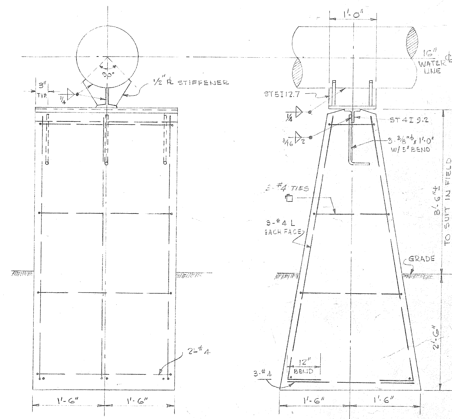
DETAIL SCALE 1"=1'-0"
