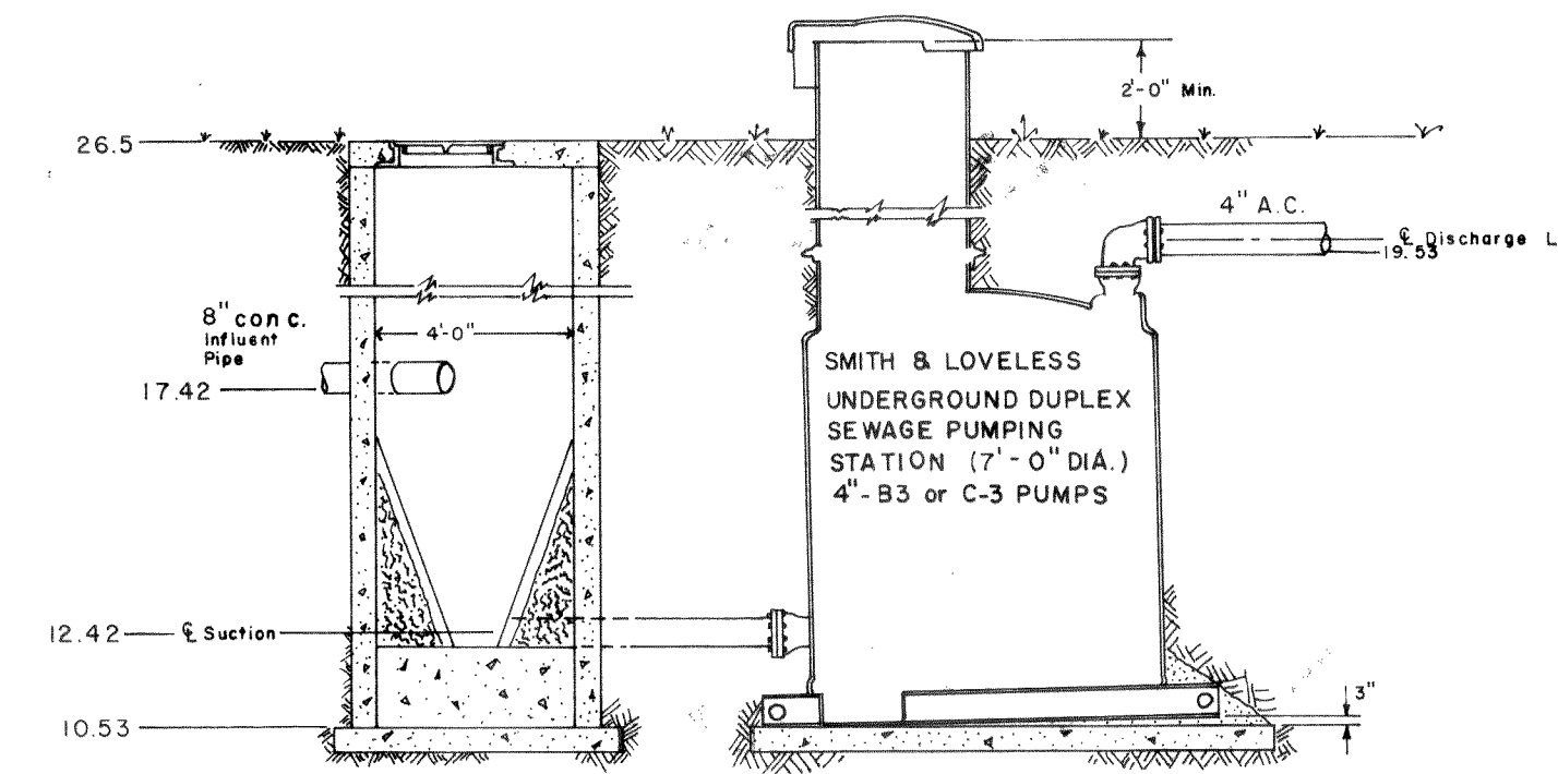
TYPICAL WET WELL LIFT STATION (CAN USE STD MANHOLE)
