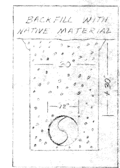
TYPICAL DITCH
